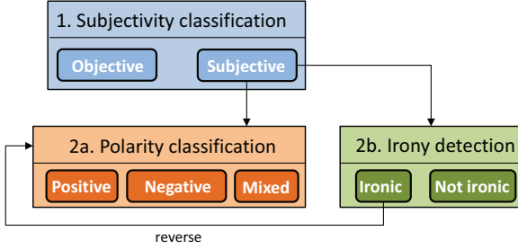
Figure 1: Hierarchical BMA.
