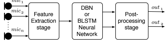
Figure 2: General block scheme of the proposed VADs.
