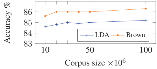
Figure 4: Clustering results
