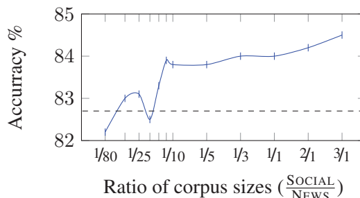
Figure 2: Oversampling results
