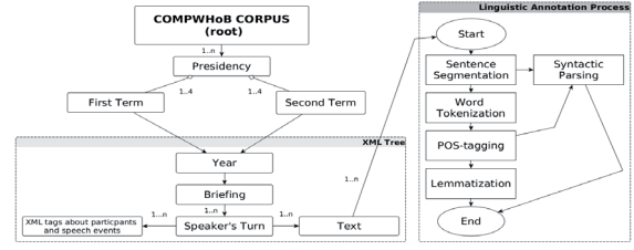
Figure 1: CompWWhoB structure and linguistic annotation process
