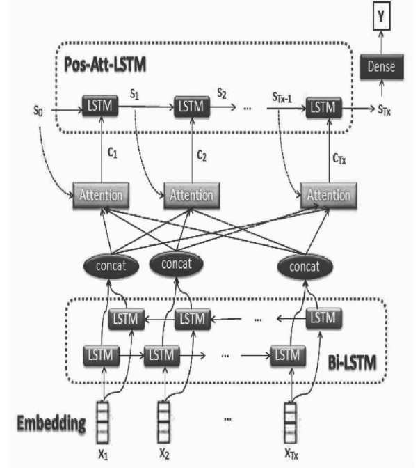
Figure 1: General architecture
