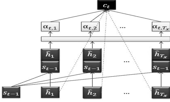
Figure 2: Attention layer
