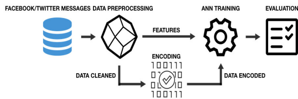
Figure 1: System architecture.
