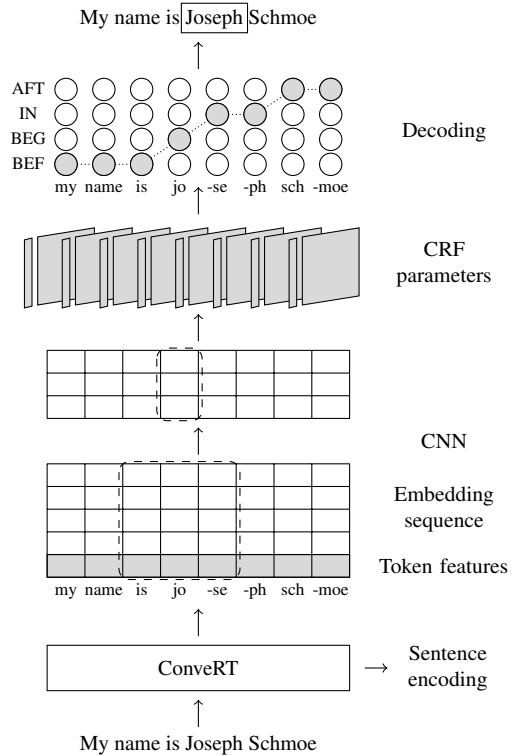
Figure 2: Span-ConveRT model architecture. Contextual subword embeddings, computed by ConveRT, are augmented with token features, and fed through a CNN. The outputs of the CNN parameterise a CRF sequence model, defining a distribution over sequence tag labellings, using the before , begin , inside , after scheme. Dashed lines denote CNN kernels.
