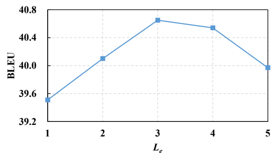
Figure 3: Results on the En⇒De validation set regarding the number L_e of graph-based multi-modal fusion layers.
