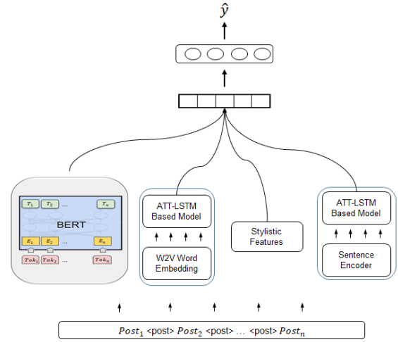
Figure 1: Representations Ensemble
