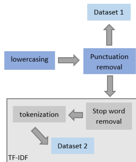
Figure 1: Data Preprocessing
