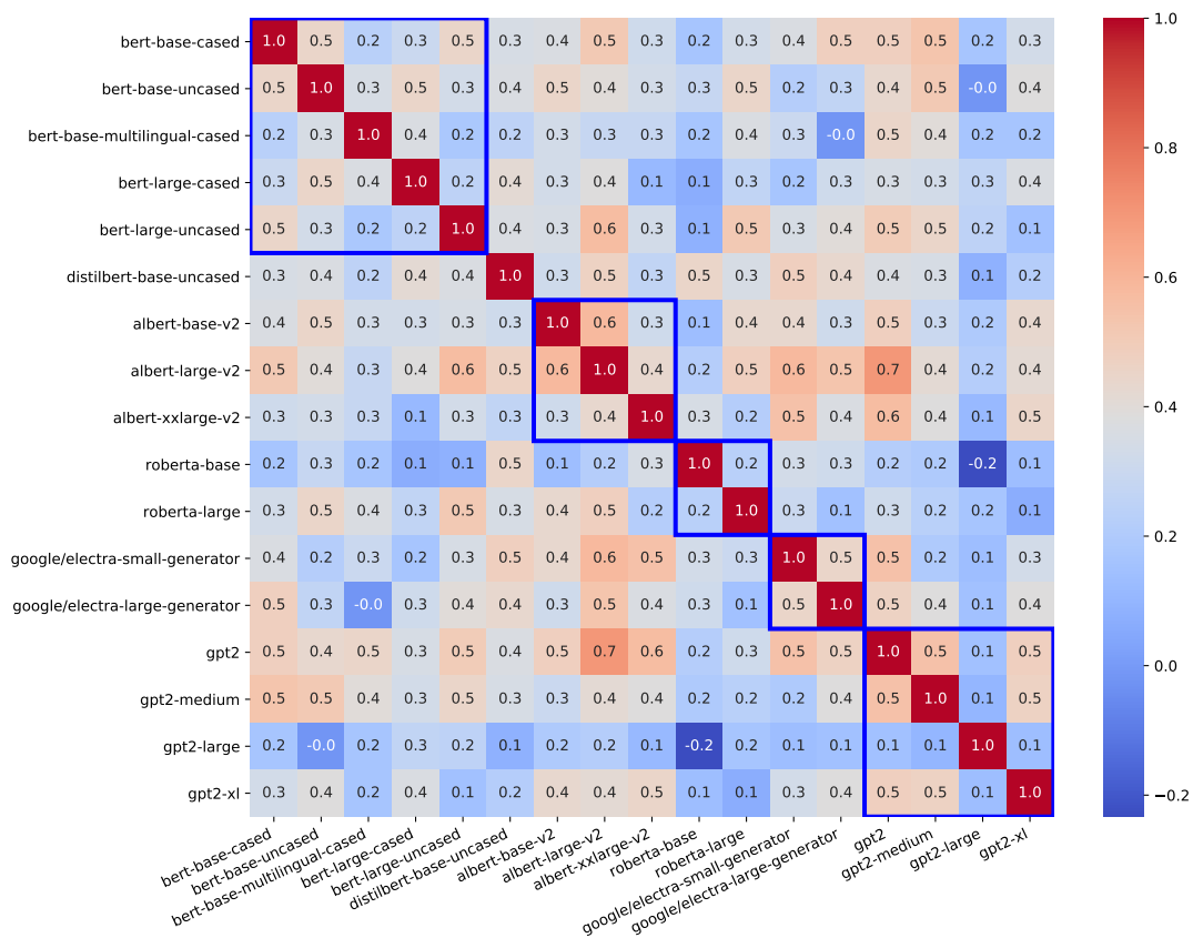
Figure 1: The heat-map of Kendall's Tau correlation coefficients between different pre-trained language models. The same type of models are in blue squares
