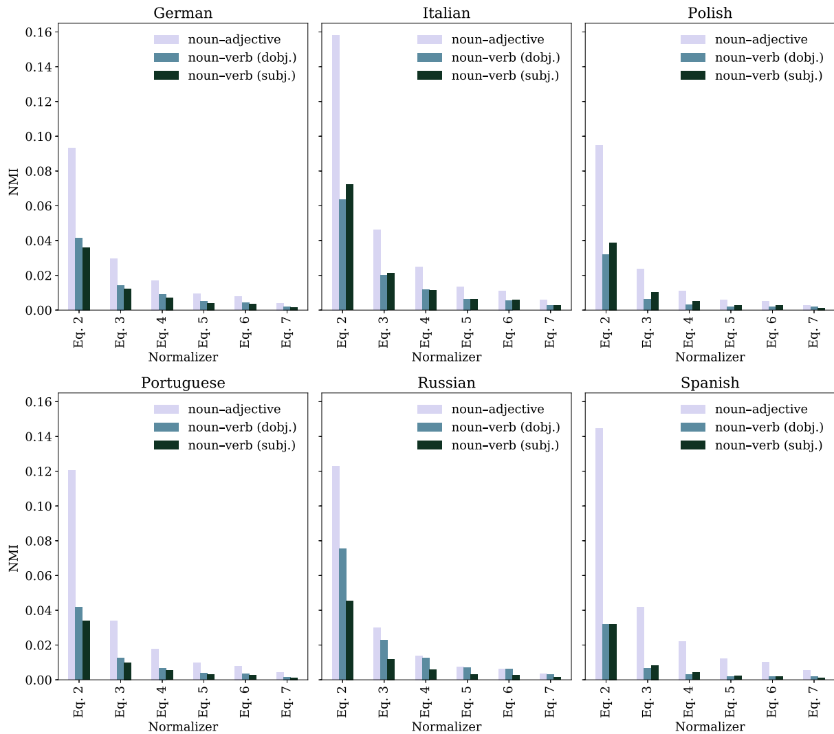
Figure 3: The normalized mutual information (NMI) between the grammatical genders of animate nouns and a) the adjectives used to describe those nouns and b) the verbs that take those nouns as direct objects and as subjects for six different gendered languages. Each subplot contains six variants of \text{NMI}(G_a^\ell, A_a^\ell) , \text{NMI}(G_a^\ell, D_a^\ell) , and \text{NMI}(G_a^\ell, S_a^\ell) —one per normalizer—for a single language \ell \in \{de, it, pl, pt, ru, es\} .
