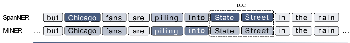
Figure 4: Visualization of attention weights over entities and context.
