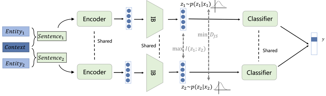
Figure 1: Visualization of MINER, where x_1 and x_2 share the same context and entity labels, while their entity words are different. z_1 and z_2 are compressed entity representations sampled by p(z_1|x_1) and p(z_2|x_2) , respectively, which are implemented by information bottleneck (IB) layer. Our method add two additional learning objectives to basic architecture. The first one is to maximize the mutual information, i.e., I(z_1; z_2) , to enhance context information and entity surface form information of z_1 and z_2 . The second objective is to minimize the Jensen-Shannon divergence, representing an upper bound of I(x_1; z_1|x_2) , aiming to eliminate task-irrelevant nuisances.
