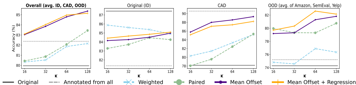
Fig. 6: SDistillRoBERTa
