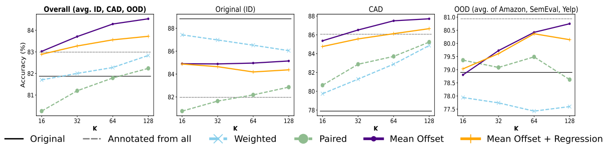
Fig. 5: SimCSE-BERT base
