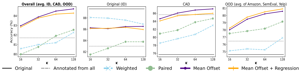
Fig. 3: SimCSE-RoBERTa large
