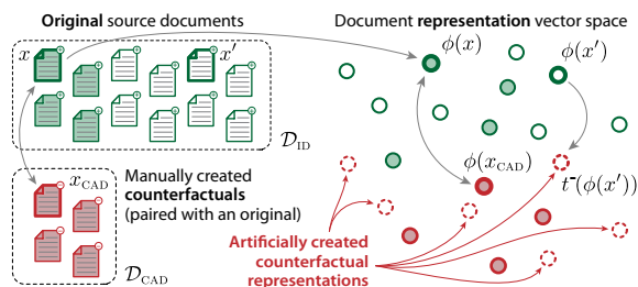
Fig. 1: We propose to generate counterfactuals in representation space, learning — from only a few manually created counterfactuals — a mapping function t to transform a document representation \phi(x) to a counterfactual one (having the opposite classification label). Illustration for positively labeled originals only.
