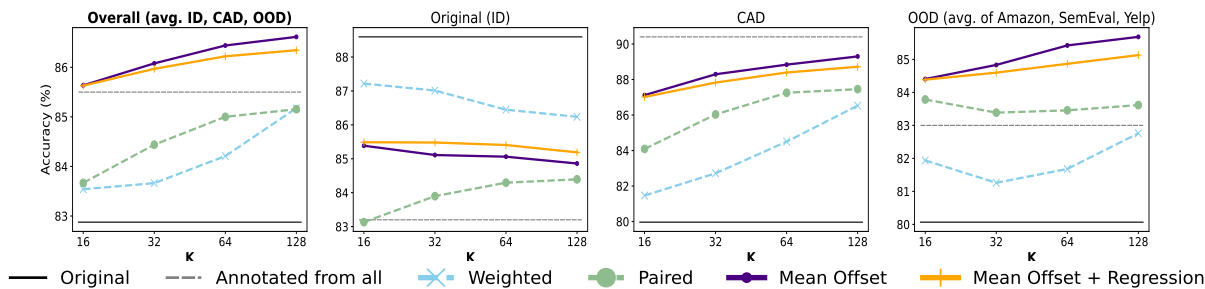
Fig. 4: SimCSE-BERT large
