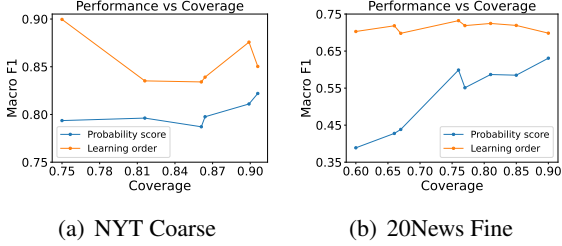
Figure 4: Macro- F_1 vs Coverage on NYT-Coarse & 20News-Fine using BERT with LOPS and Probability score based selection.
