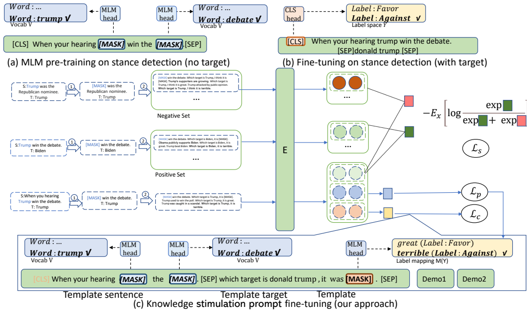
Figure 1: An illustration of (a) masked language model (MLM) pre-training, (b) fine-tuning, and (c) our proposed knowledge stimulation prompt fine-tuning approach.
