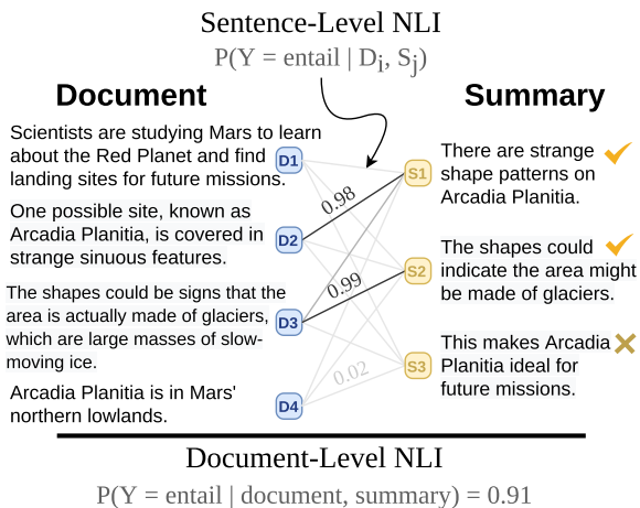
Figure 1: Example document with an inconsistent summary. When running each sentence pair (D_i, S_j) through an NLI model, S_3 is not entailed by any document sentence. However, when running the entire (document, summary) at once, the NLI model incorrectly predicts that the document highly entails the entire summary.
