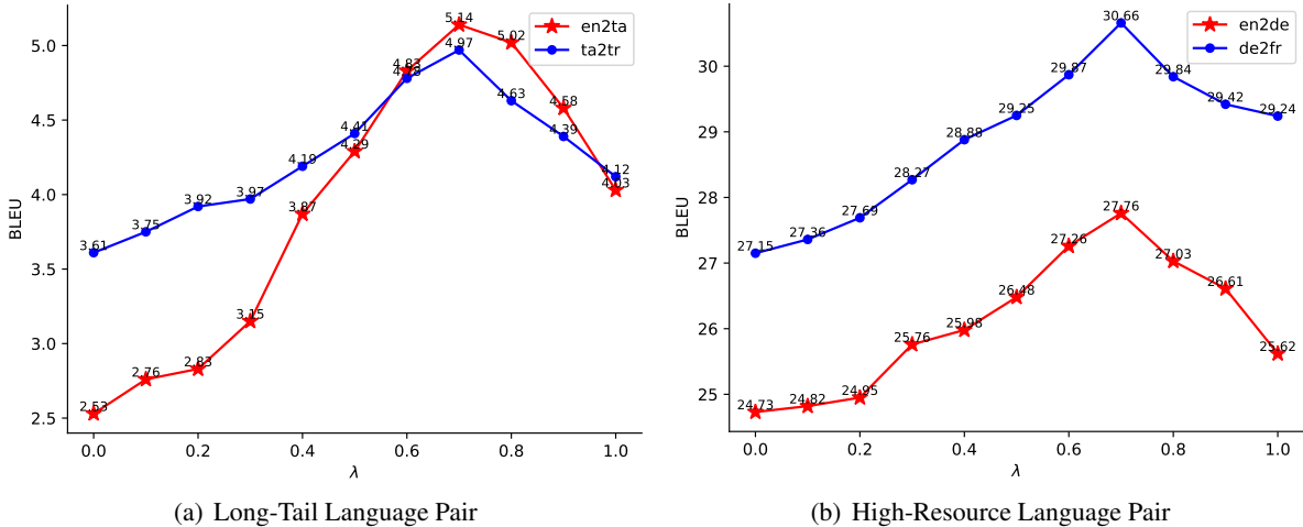
Figure 4: The effect of different \lambda
