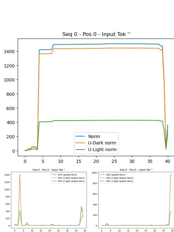
Figure 9: (Top) The composition of the RS of the BoS token for LLaMa2 13B as a function of the layer. (Bottom left) The norms of the contribution of MLP layers to the BoS RS. (Bottom right) The norms of the contribution of Multi-Head Attention components to the BoS RS.
