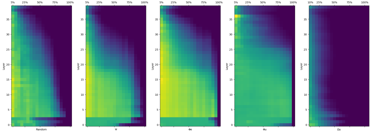
Figure 20: NLL filtering of MLPs in LLaMa2 13B on a sample of code from the DeepMind Code Contest dataset.
