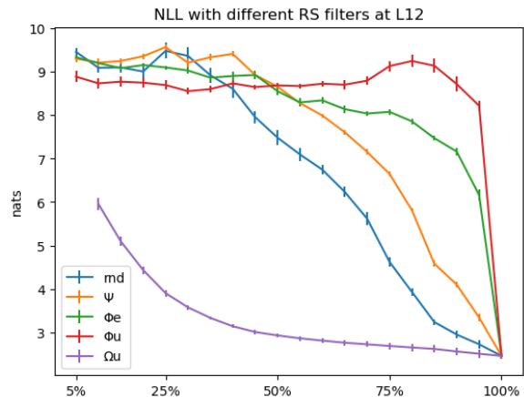
Figure 13: NLL by number of retained dimensions when applying different spectral filters at L12. Error bars indicate three standard deviations over five repeats with samples from the same source and of the same approximate size as ccnet-405.
