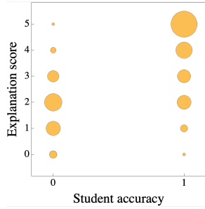
Figure 2: In student models, (human-annotated) explanation scores E_{SC} vary greatly within cases where models get the answer right (accuracy = 1) or wrong (accuracy = 0). Even when a model gets the answer correct, its reasoning chain can contain varying degrees of flaws. On the other hand, when a model is incorrect in its answer, it could still make some valid points.
