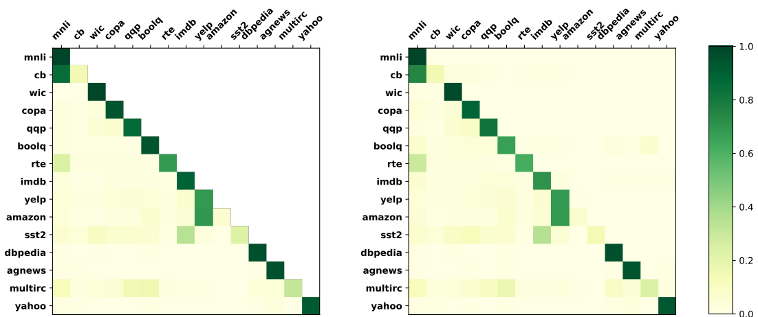
Figure 12: Visualization on shared attention of SAPT-LoRA on the Long Sequence benchmark during the training (left) and testing time (right).
