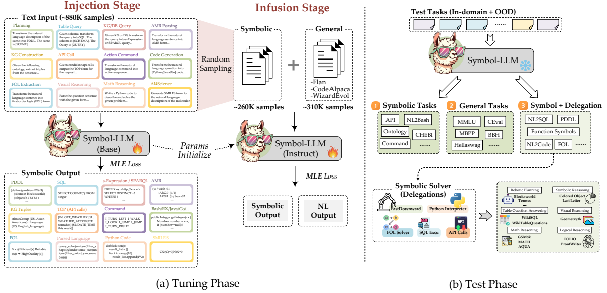
Figure 2: Overall pipeline of Symbol-LLM. (a) is two-stage tuning framework, Injection stage and Infusion stage. (b) is the test phase with comprehensive settings, symbolic tasks, general tasks, and downstream tasks under the Symbol+Delegation paradigm.
