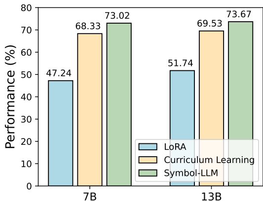
Figure 9: Comparison between different tuning design choices.
