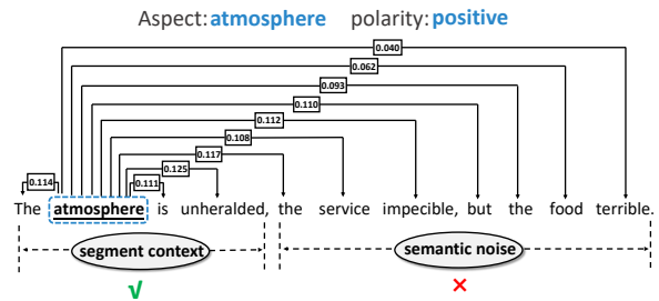
Figure 1: The attention weight of the aspect word "atmosphere" in relation to other words in the sentence. "x" refers to noise information for "atmosphere".
