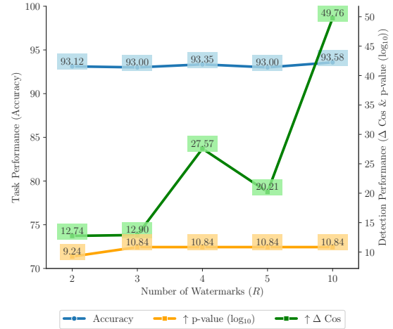
Figure 7: The impact of GS extension on WARDEN for SST2 dataset. The observations are in line with normal WARDEN (Figure 6) results with the only difference being stronger metrics.
