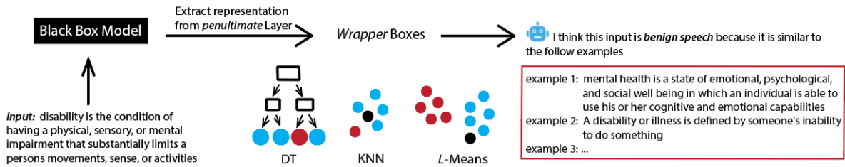
Figure 1: Three wrapper boxes illustrated for toxic language detection (Hartvigsen et al., 2022). Red and blue dots denote harmful vs. benign speech. Smaller dots represent examples, while larger dots represent clusters (e.g., DT leaf nodes). A neural model’s penultimate layer provides the feature representation for the white wrapper boxes. Our results show that classic models can achieve comparable performance to the underlying neural models while also providing intuitive, example-based explanations (described in Section 4).
