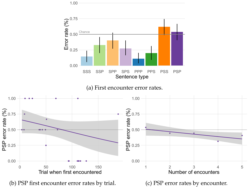
Figure 6 Human error rates on inner/embedded dependencies from Lakretz et al. (2021), reanalyzed to explore learning effects. Note that these plots are after the humans have completed their training phase. (a) Performance on all structures the first time they are encountered after training. Humans do not appear to perform better than chance on the most difficult structures. (b) Performance on the key PSP structure when it is first encountered, as a function of trial—a proxy for experience on related structures. (c) Performance on the PSP structure, with the target grammar violation, as a function of the number of times it has been encountered. The results are suggestive of a learning effect, but are not conclusive due to the small sample size. (Points/bars are aggregates across subjects—in panel b, all subjects who first encountered that structure at that trial. Error bars in panel a are bootstrap 95%-CIs; lines/ranges in panels b-c are logistic regression fits.)
