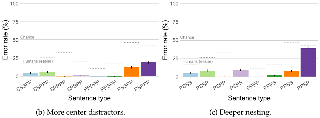
Figure 4 Chinchilla (70B), with the same eight-shot prompts, evaluated on more challenging conditions. (a) The modifications to the tasks—either nesting the sentence more deeply (top), or inserting more center distractors (bottom). (b) Adding two more distractor plural prepositional phrases in the center does not substantially change the error rates. (c) Increasing the embedding depth, by prepending an additional plural prefix does increase error rates in the most challenging condition—however, the model still performs better than humans do in easier conditions, indicated as dashed lines. (The dashed lines show human performance in the hardest conditions that Lakretz et al. (2021) evaluated with humans; the conditions we evaluate the model on here are alterations intended to make the task even more difficult, especially in the PSP condition. Error bars are bootstrap 95%-CIs across task examples and three prompts.)
