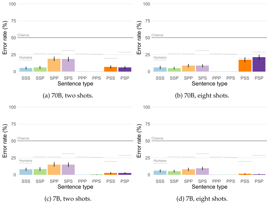
Figure B3 Both the 70B (Chinchilla, top) and 7B (bottom) parameter model also perform well at the outer agreement task. With either a two-shot (a,c) or eight-shot prompt (b,d), both models perform better than humans in most or all conditions. Intriguingly, the larger model actually makes more errors than the smaller; but in that sense its performance is more like the humans. The longer prompt also shifts the error patterns for the large model. Overall errors remain fairly low compared to the humans, across all models and prompts. (Error bars are bootstrap 95%-CIs. Dashed lines show human performance, from Lakretz et al. 2021.)
