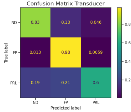
(b) RNN-T-based classifier with hidden size 640 trained on distilled features from layer 16 (index 15 in F1,DTW plots).
