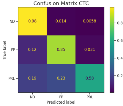
(a) CTC-based classifier with hidden size 640 trained on distilled features from layer 18 (index 17 in F1,DTW plots).
