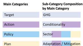
Figure 1: Classification Schema
