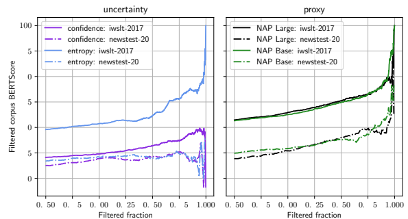
Figure 3: Measuring T5 Large performance on a filtered dataset when removing the worst examples according to some metric.
