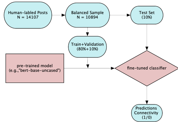
Figure 1: Pipeline of fine-tuning a BERT classifier for detecting connective language
