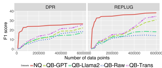
Figure 2: QB-Trans can replace NQ in training QA system and achieve accuracy close to NQ training system. DPR: As expected, QB-TRANS without any NQ data comes within 5 points of a model trained on NQ. Training on the full QB-TRANS and evaluating it produces the highest F1 score system with DPR. This does better than transformations created by prompting a GPT and LLAMA. REPLUG: Again, QB-TRANS without any NQ data comes within 7 points of a model trained on NQ.
