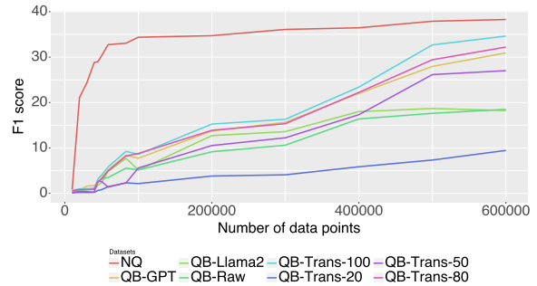
Figure 6: QB-Trans can replace NQ in training QA system and achieve accuracy close to NQ training system. As expected, QB-Trans-100 without any NQ data comes within 5 points of a model trained on NQ. Training on the full QB-Trans and evaluating it produces the highest accuracy system with DPR. However, the percentage of that dataset from our systematic conversion ( QB-Trans-80 ) reaches a substantial fraction of the accuracy. This does better than conversions created by prompting a LLM.
