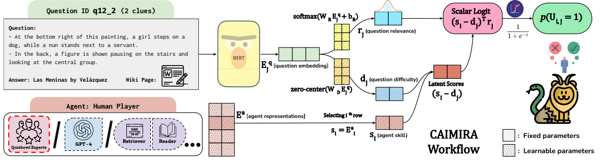
Figure 3: The CAIMIRA workflow. It predicts the probability of agent- i correctly answering question- j using a model in Eq. (3). Here, the question’s raw relevance r_j' and raw difficulty d_j' are multidimensional and computed by learnt linear transformations over the question embedding E_j^q (§ 3.3), and the agent skill s_i is extracted from a learnable agent embedding matrix E^a . r_j is a probability distribution computed from the raw reference r_j' and improves the interpretability of the multidimensional model (§ 3.1); d_j is achieved by zero centering of the raw difficulty d_j' , which addresses the non-identifiability issue of s_i and d_j in (s_i - d_j) (§ 3.2).
