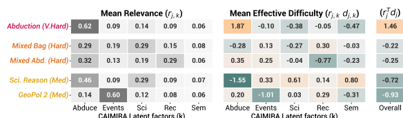
Figure 10: Heatmaps of mean relevance r_{j,k} and mean effective difficulty d_{D,\mu_k}^{(e)} of selected question clusters (on effective difficulty) across the five latent factors ( k ).
