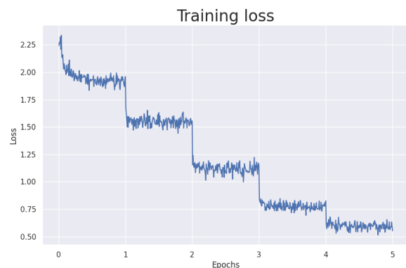
Figure 3: Training loss over time for Mistral-7B.
