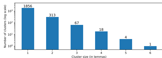
Figure 2: Distribution of cluster size (in number of lemmas) obtained by the Bi-level Agglo system.
