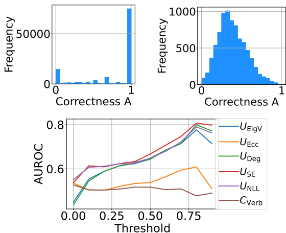
Figure 4: Top: Rouge-L correctness distributions of GPT-3.5-turbo on the TriviaQA (left) and Meadow (right) benchmarks. Bottom: AUROCs of assessed measures for GPT-3.5-turbo on Meadow, with Rouge-L correctness and various thresholds.
