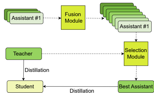
Figure 1: MTA4DPR Framework. MTA4DPR transfers knowledge from the teacher to the student with the help of the best assistant. The Fusion Module is used to generate fused assistants from the original assistants, and the Selection Module is used to select the best assistant among all original and fused assistants. The dotted arrows indicate that the corresponding procedures are not involved in the backpropagation of the training.
