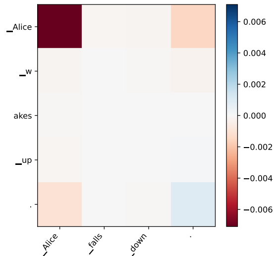
Figure 1: Attribution scores on individual tokens in the final layer of our StoryEmb model are shown as a delta from the E5 model. Negative scores indicate less contribution to the similarity in the StoryEmb model. In the example, it seems clear that less emphasis is placed on named entities.
