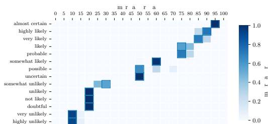
(e) Gemini
