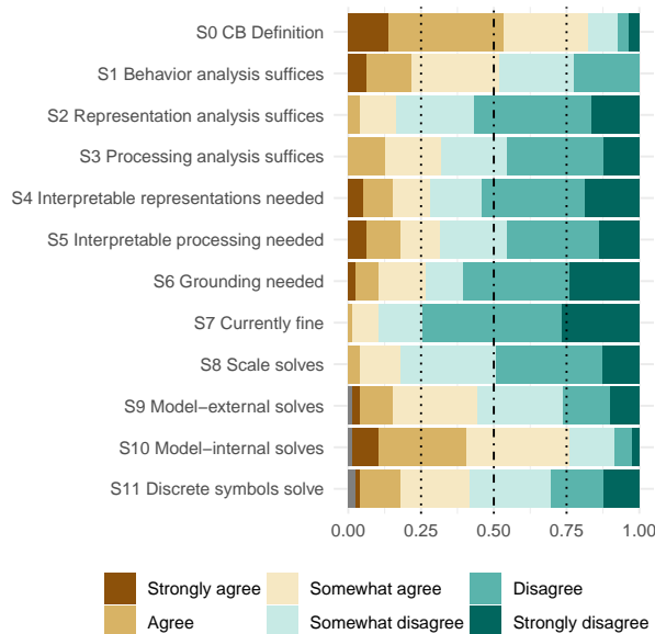
Figure 1: Overview of survey responses. We find consensus (i.e. \sim 75\% + concordance on “agree” or “disagree”) for 7 of the 12 surveyed claims.
