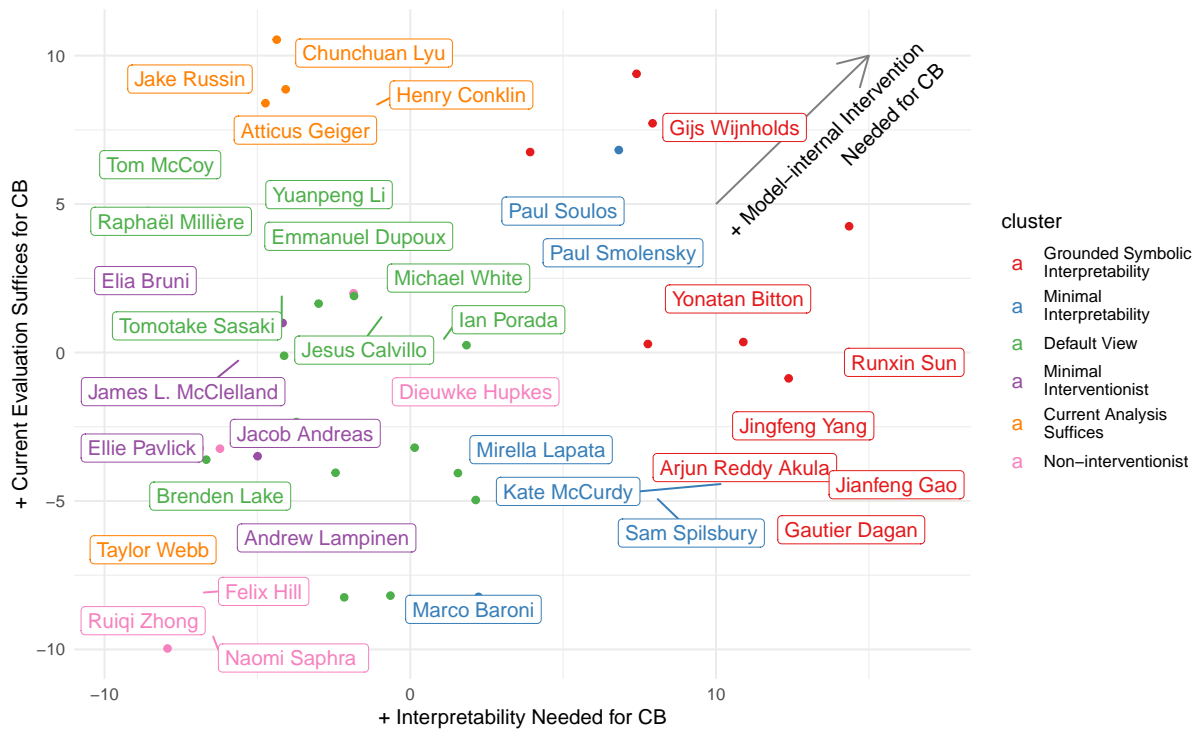
Figure 3: Logical geography of CB survey responses, inspired by Dennett (1986) . Individual respondents are projected to a two-dimensional location using principal component analysis and colored based on cluster (cf. Appendix B). Points represent participants who did not give permission to use their name. Axis labels reflect our loose interpretation of the principal components.
