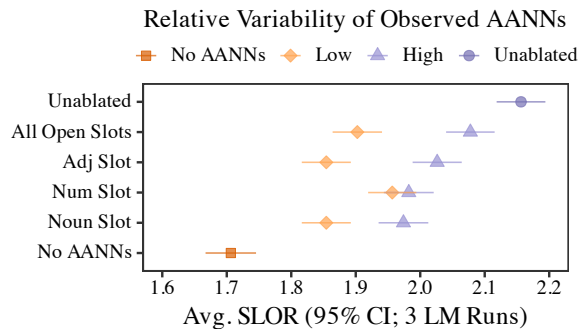
Figure 5: SLORS on AANNs from Mahowald (2023) for LMs trained on BabyLM with low and high variability in the open slots of the observed AANN instances. When models are presented with higher variability for a given slot, the construction is typically learned better.
