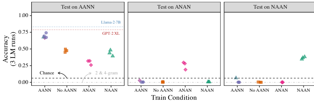
Figure 2: Accuracies on tests for AANN and its counterfactuals (ANAN and NAAN), achieved by LMs trained on BabyLM with various AANN-manipulations (AANN as is, NO AANN, ANAN, NAAN). \blacklozenge and \blacktriangle under the AANN training condition are cases where training data was polluted by randomly replacing 300 AANNs with ANANs and NAANs, respectively, in order to assess the impact of an imperfect AANN detection system. The dashed line represents chance performance (6.25%) and the dot-dashed line represents accuracies for 2- and 4-gram LMs trained on BabyLM. Accuracies for GPT-2-XL (Radford et al., 2019) and Llama-2-7B (Touvron et al., 2023) are computed using log-probabilities , since unigram frequencies were unavailable for these LMs’ corpora.
