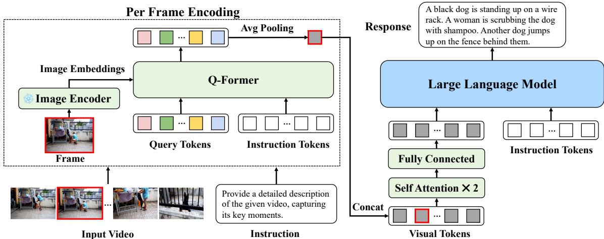
Figure 1: UNICORN framework using video paragraph captioning as an example. We encode each video frame separately and concatenate their resulting visual tokens to represent the video. We highlight the encoding process of one frame in red. All modules are instruction-tuned with the language modeling loss except the image encoder.
