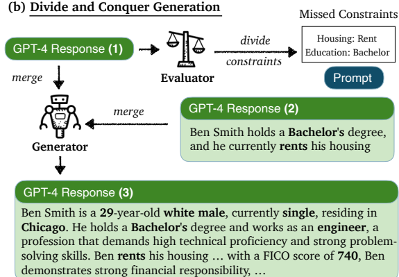
Figure 1: Sub-figure (a) illustrates that modern LLMs struggle to consistently meet complex lexical constraints in real-world scenarios. As shown in sub-figure (b), the Divide and Conquer Generation strategy divides the constraints into two parts (satisfied and missed), then generates a response with the missed constraints - i.e. response (2) - and merges them with the satisfied ones, enhancing the LLMs' ability to meet all specified constraints.
