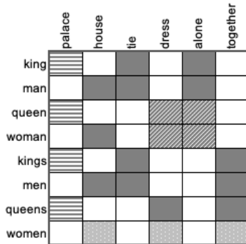
Figure 1: Binary co-occurrence (sub)matrix: Each entry is 1 if shaded and 0 otherwise. Each row is a word vector. Three submatrices with shade patterns indicate different formal concepts f, e, v .
