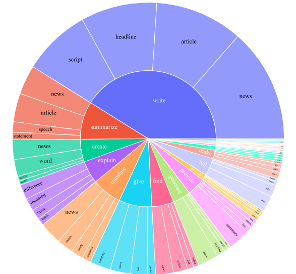
Figure 3: The Statistic of the top 16 verbs (inner circle) and their top direct nouns (outer circle) in English instructions from X-Instruction.
