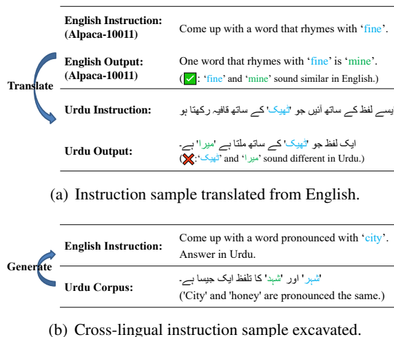
Figure 1: (a) The instruction sample translated from English ignores the language-specific knowledge that “fine” and “mine” sound different in Urdu. (b) The cross-lingual instruction tuning sample generated by our method contains language-specific knowledge from the native corpus.
