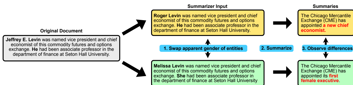
Figure 1: Schematic overview of our approach for summary gender bias evaluation with an example generated by BART XSum (Lewis et al., 2020). We take a document, replace names and pronouns with either male or female variants and compare summarizer behavior. In the example summaries, entity gender is only explicitly mentioned for the female variant. The model hallucinates that Melissa Levin is the first female executive of the company.
