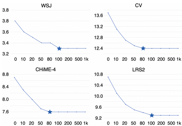
Figure 4: WER (%) results of utilizing different numbers of validation samples for prior estimation. The minimum required amount to obtain the best performance is highlighted in the star mark.
