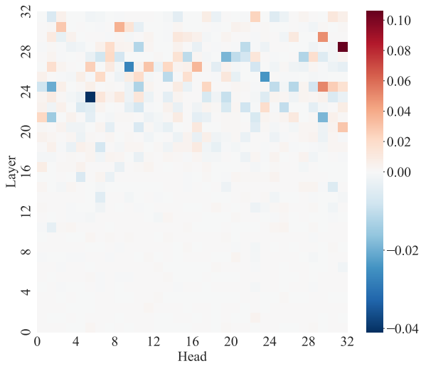
Figure 21: Memory Heads of OPT-2.7B.
