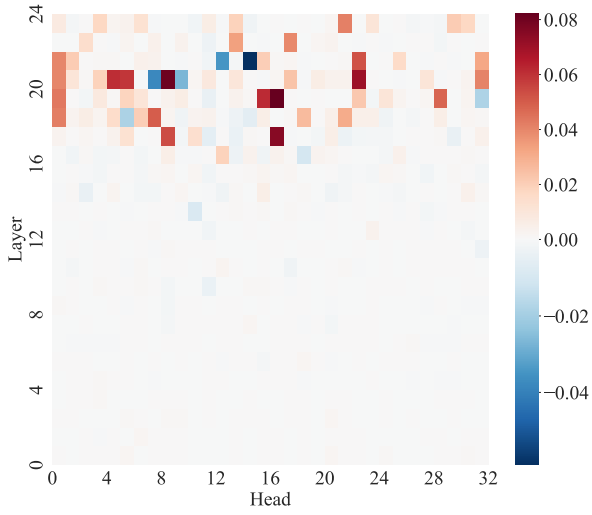
Figure 20: Context Heads of OPT-1.3B.
