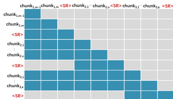
Figure 1: The modified attention mask is illustrated in the figure, where cell (r, c) signifies whether token r can attend to token c . chunk_{2,1} represents the first token of the second chunk, with similar patterns for other chunks.
