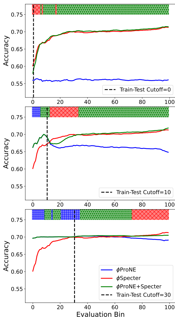
Figure 10: Hybrid Forecast Accuracy (with 5-point Moving Average) for \phi_{\frac{P_\tau}{S}} with ProNE-S (0) , (10) , (30) and Specter. The color bars indicate which line has the best accuracy. Differences between bars suggest the policy for combining text and context depends on the size of the training set ( t ) and forecasting horizon ( h ).
