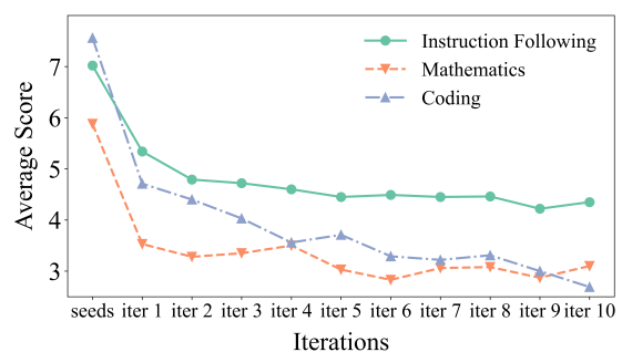
Figure 3: The change in the average score during the iterative search process for the three tasks.
