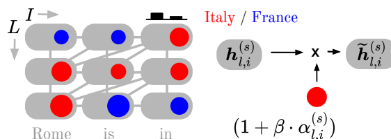
Figure 1: We show that it is often sufficient to scale a few influential activation vectors h_{l,i}^{(s)} for a model to favor one answer token over another token. This could be the MLP output at layer l for token position i . We learn multiplicative scalars, \alpha_{l,i}^{(s)} , using gradient-based optimization. These correspond to interpretable interventions that generalize to test set prompts while relying on fewer parameters than additive steering vectors.
