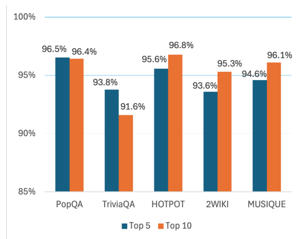
Figure 4: The ratio of contents extracted by Refiner that are exactly originate from respective document chunks under various top retrieval settings and tasks.
