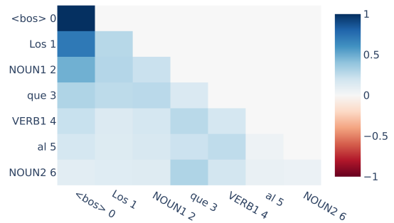
Figure 21: L13H7 average attention patterns (output-value weighted) across the Spanish dataset.
