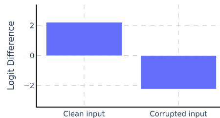
Figure 9: Logit Difference on clean and corrupted inputs. Spanish dataset.
