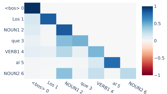
Figure 22: L17H4 Average attention patterns (output-value weighted) across the English dataset.
